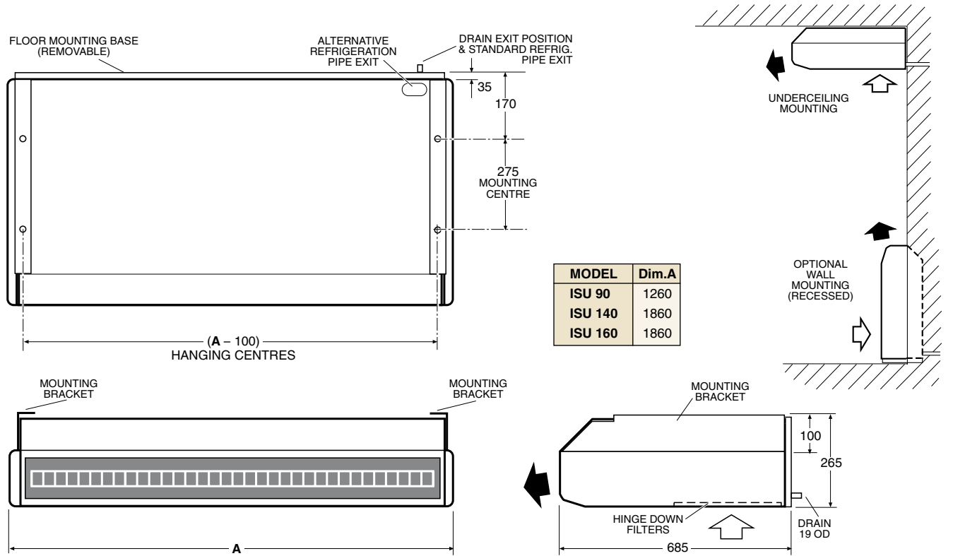
Fig. 1 ISU 90, 140, 160 Underceiling/Console
