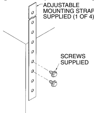
Fig. 4 Strap Mounting
