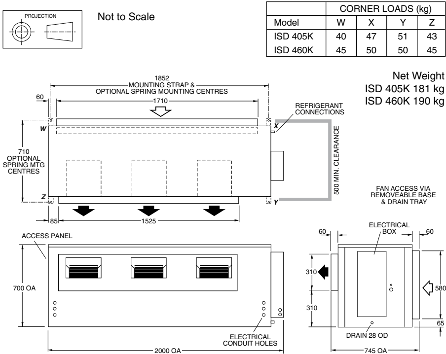
Fig.1 Dimensions (mm)
